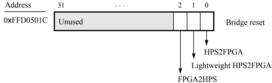
Figure 7. FPGA bridge reset register.
