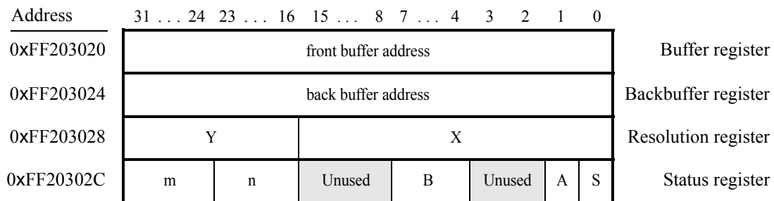
Figure 38. Pixel buffer controller registers.
